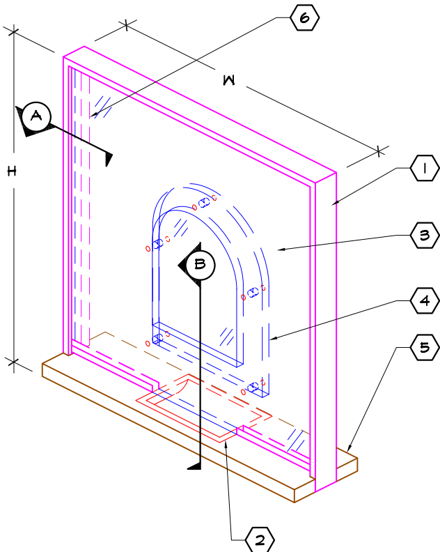
ISOMETRIC
